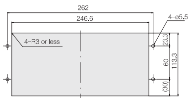
(Panel cut-out diagram)
