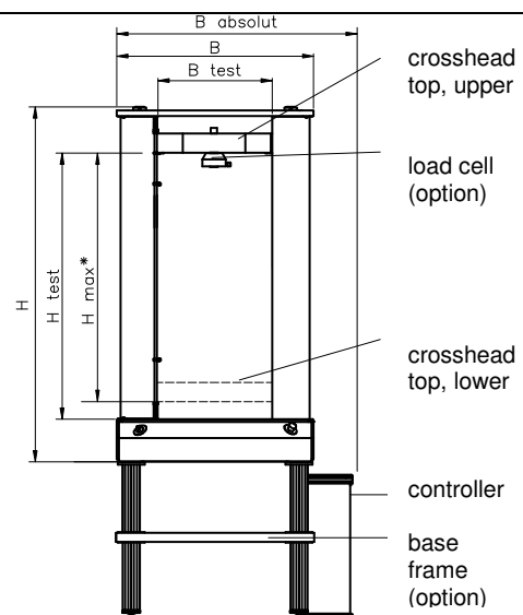
View universal testing machine with dimensions
