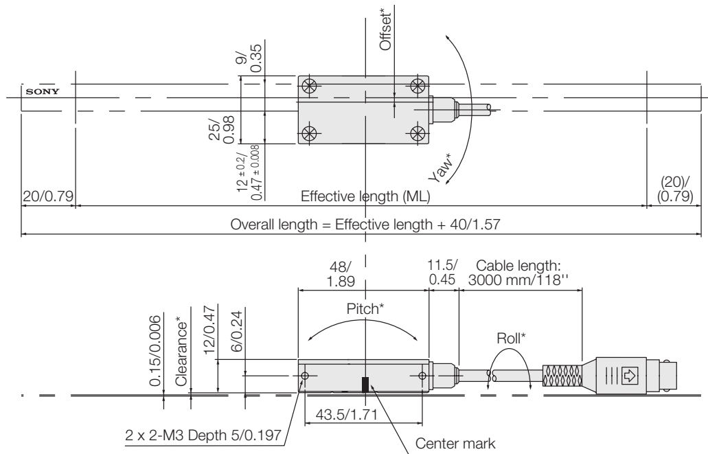
PL101-RH (IP67 Type)
