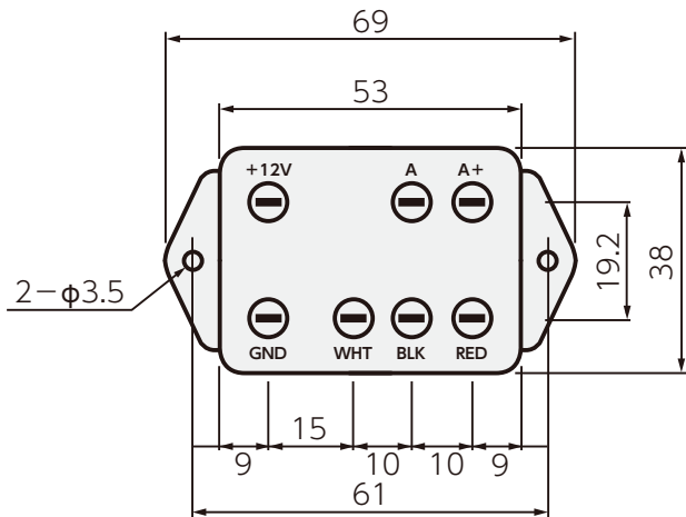
Detector PD-10
