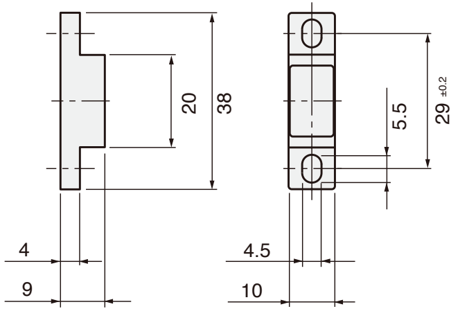
Magnet PG-104(PG-10)
