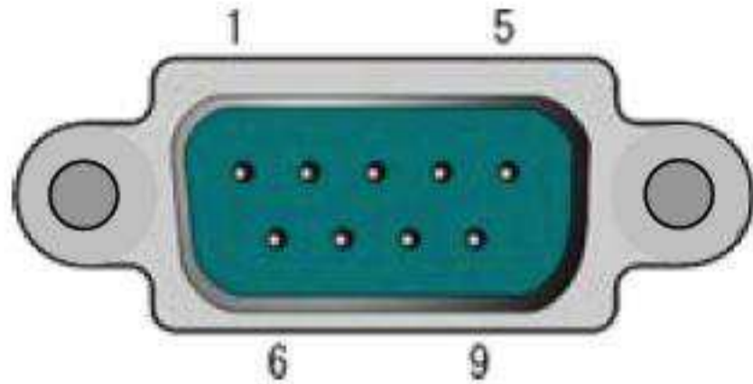
Output connector of SJ700A
