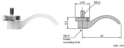
DZ-581 Measuring force balancer (for DK110, DG110B)
