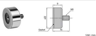
DZ-123 Feeler (for DK Series, DG805BL/810B/810BL)
